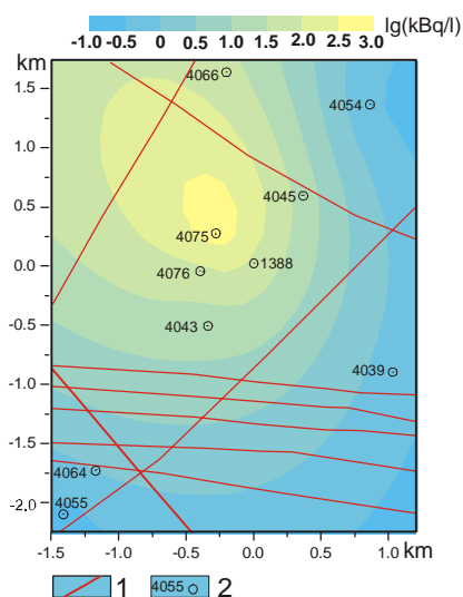
Fig. 1. Scheme of ^3\text{H} distribution (max.values, lg(kBq/l; 1 – fault; 2 – well and its number).
