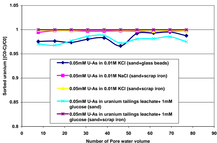
Fig. 10. Removal effectiveness of 0.05mM uranium under 0.05mM arsenic, iron and micro-organisms influence in 0.01M NaCl, 0.01M KCl at pH 4.5 and Schneckenstein Uranium Tailings PNP9 upgraded to 0.05mM uranium-arsenic concentration at near neutral pH.
